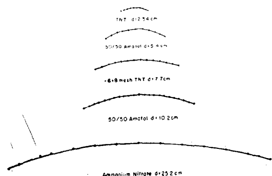
Figure 5.6e Representative plots of reduced data showing sphericity of wave front
